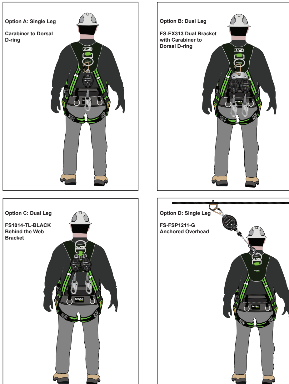
FIGURE 1 - HARNESS CONNECTIONS
