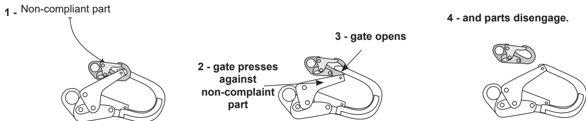
FIGURE 5 - UNINTENTIONAL DISENGAGEMENT
