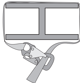
FIGURE 13 - TIE BACK ANCHORING
