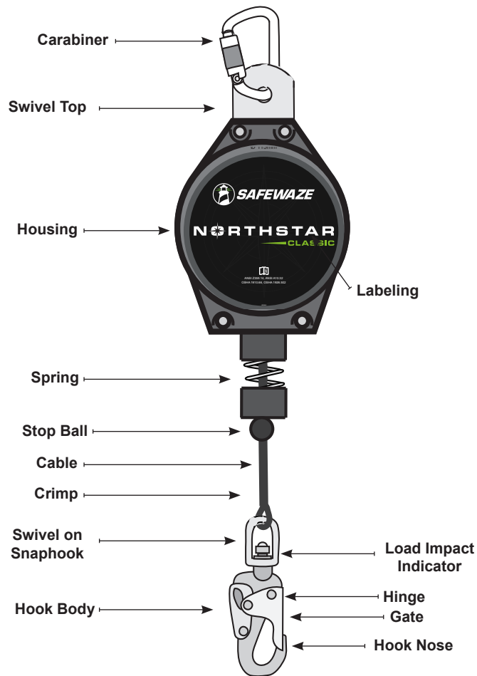
FIGURE 17 - INSPECTION DIAGRAM
