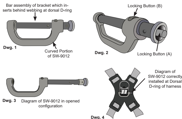
FIGURE 8 - SW-9012 DUAL BRACKET INSTALLATION
