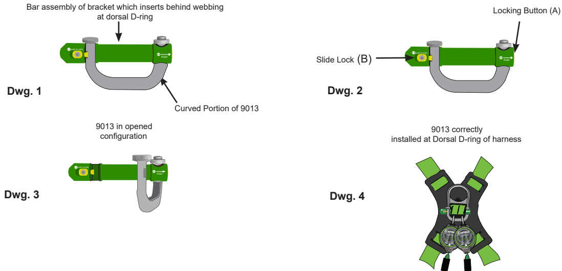
FIGURE 10 - 9013 DUAL BRACKET INSTALLATION
