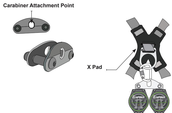
FIGURE 9 - CARABINER W/DUAL BRACKET INSTALLATION
