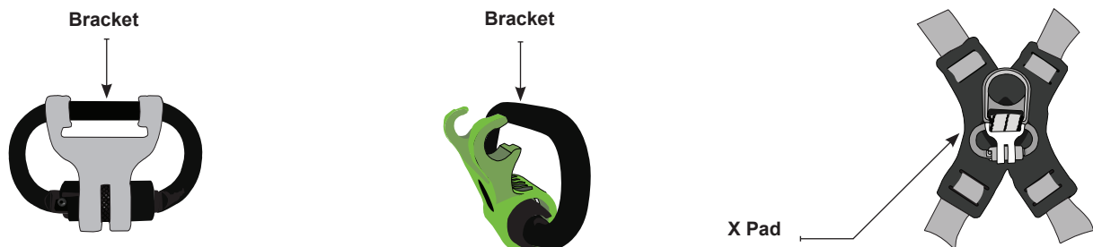
FIGURE 7 - BEHIND THE WEB BRACKET INSTALLATION
