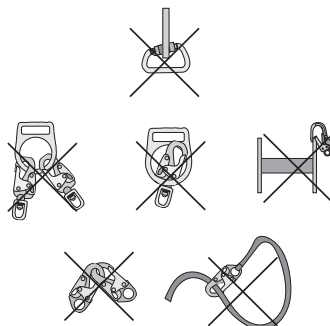
FIGURE 6 - INAPPROPRIATE CONNECTIONS
