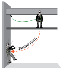
FIGURE 2 - SWING FALLS
