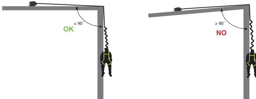
FIGURE 3 - LE ANCHOR POINT ILLUSTRATION
